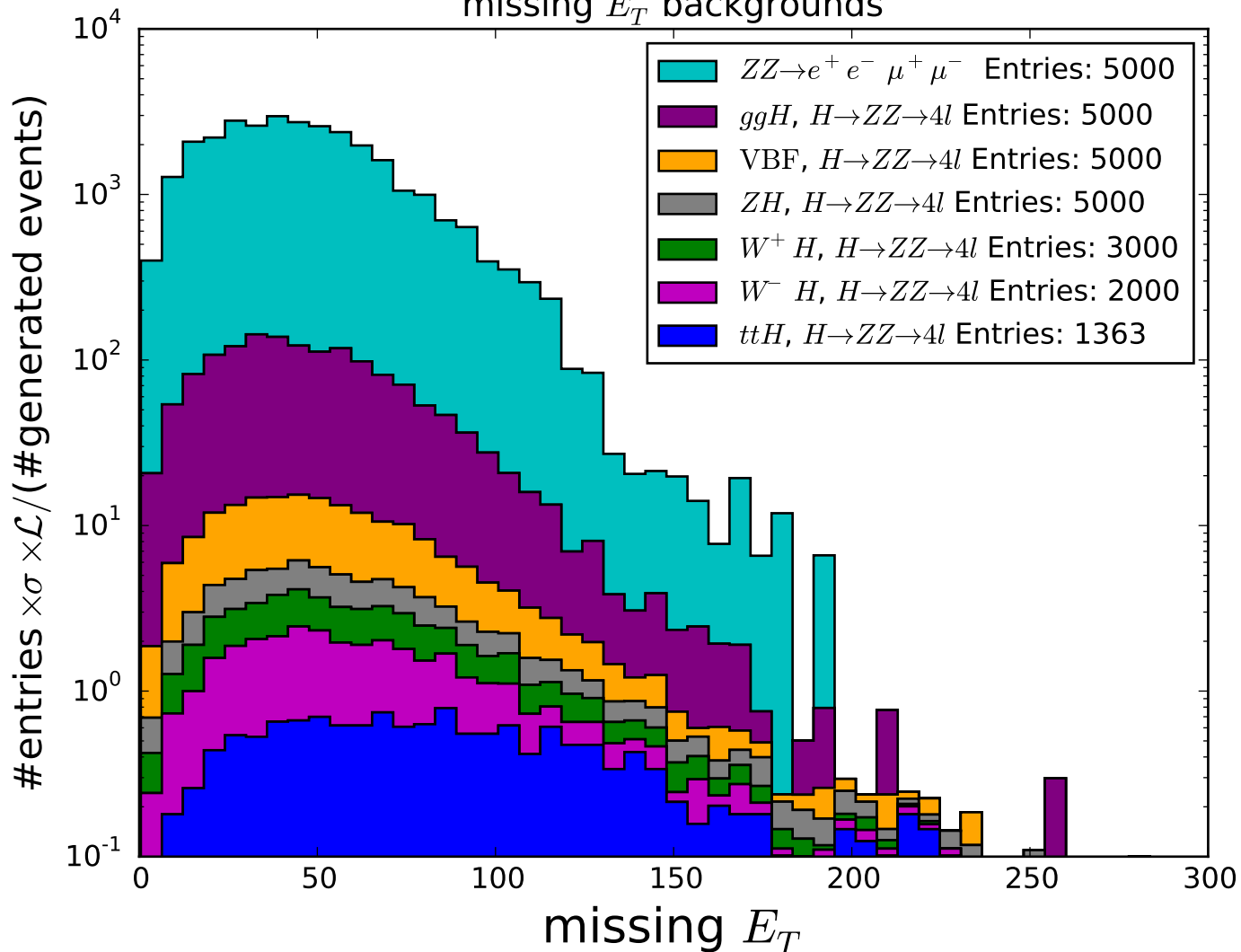
missing E_T backgrounds
