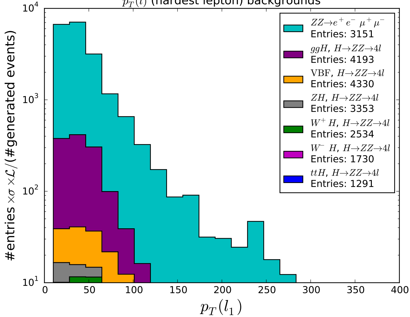
p_T(l) (hardest lepton) backgrounds
