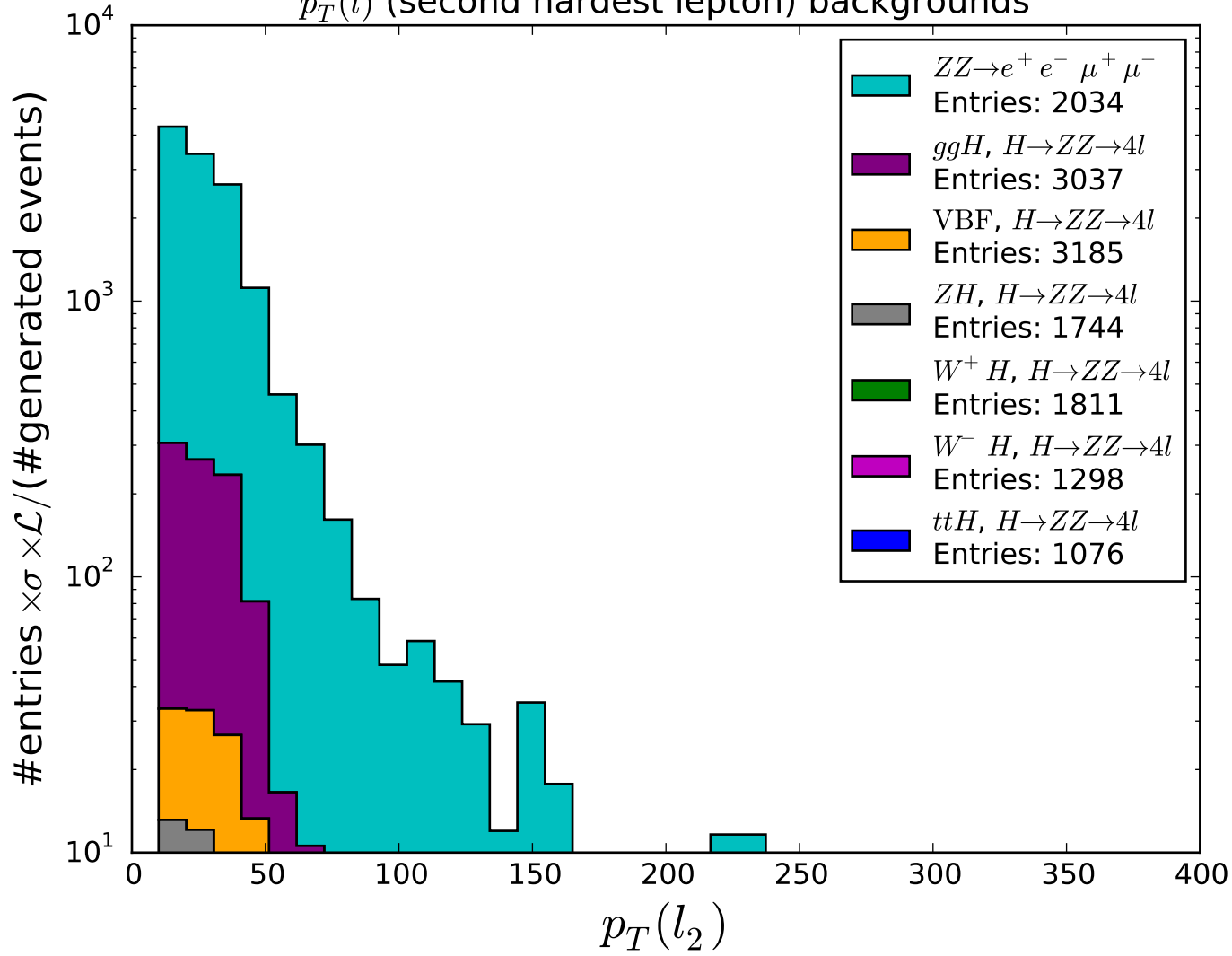
p_T(l) (second hardest lepton) backgrounds
