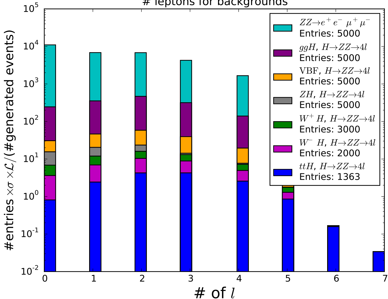
# leptons for backgrounds
