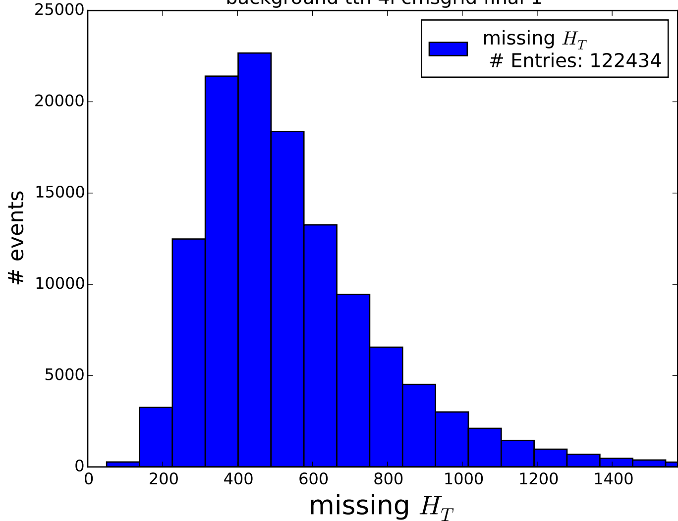
background tth 4l cmsgrid final 1
