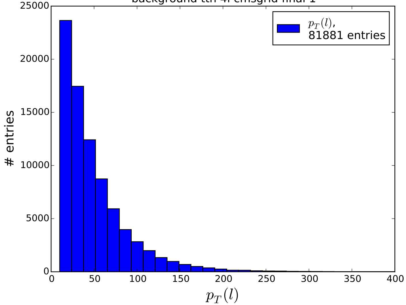
background tth 4l cmsgrid final 1
