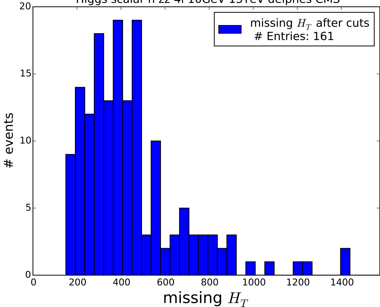
Higgs scalar h zz 4l 10GeV 13TeV delphes CMS
