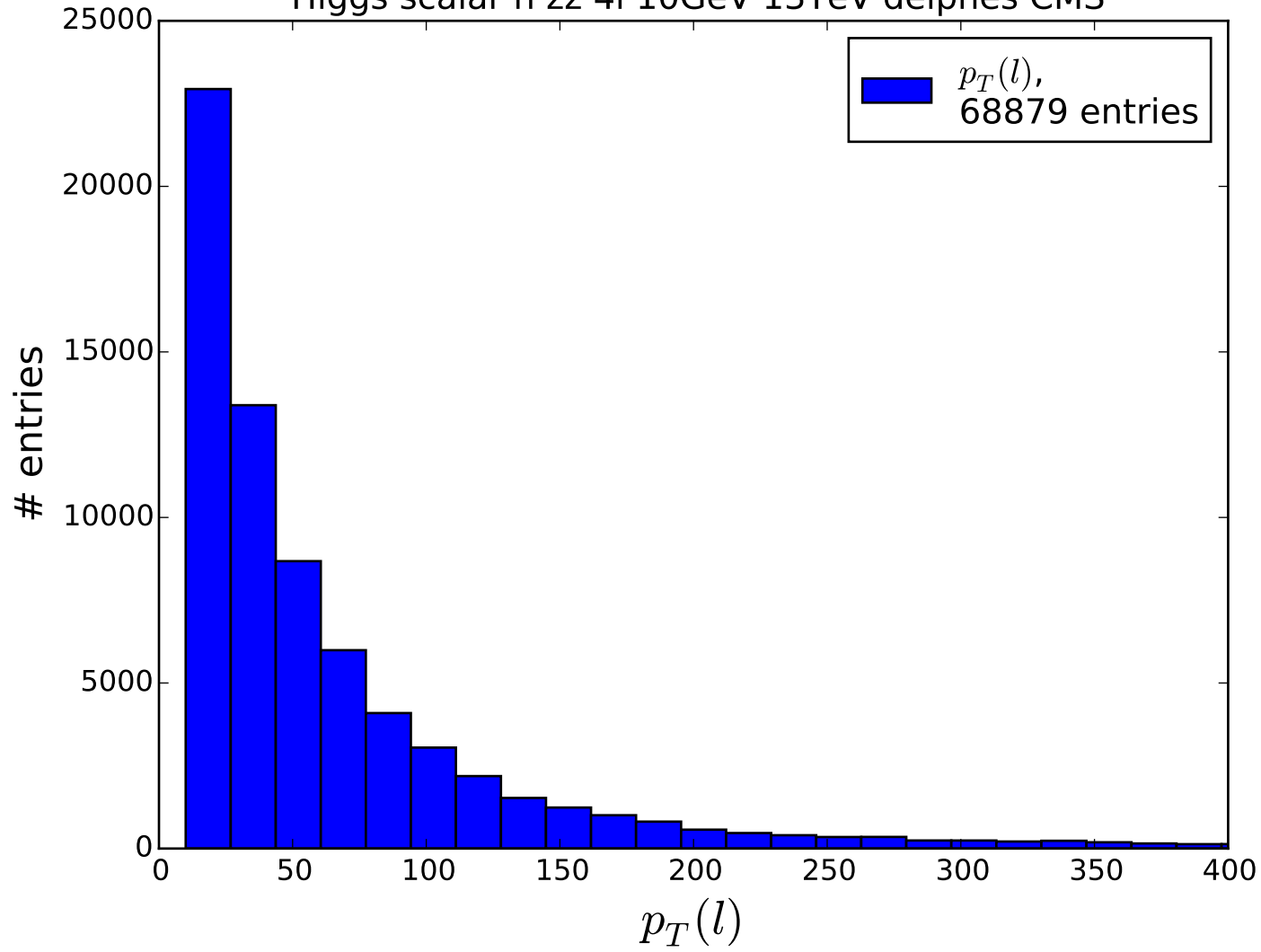
Higgs scalar h zz 4l 10GeV 13TeV delphes CMS
