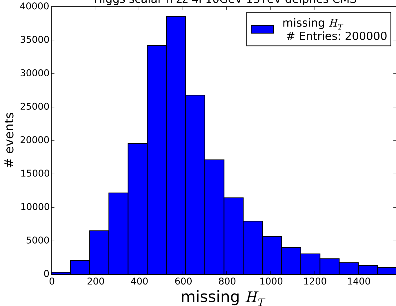
Higgs scalar h zz 4l 10GeV 13TeV delphes CMS
