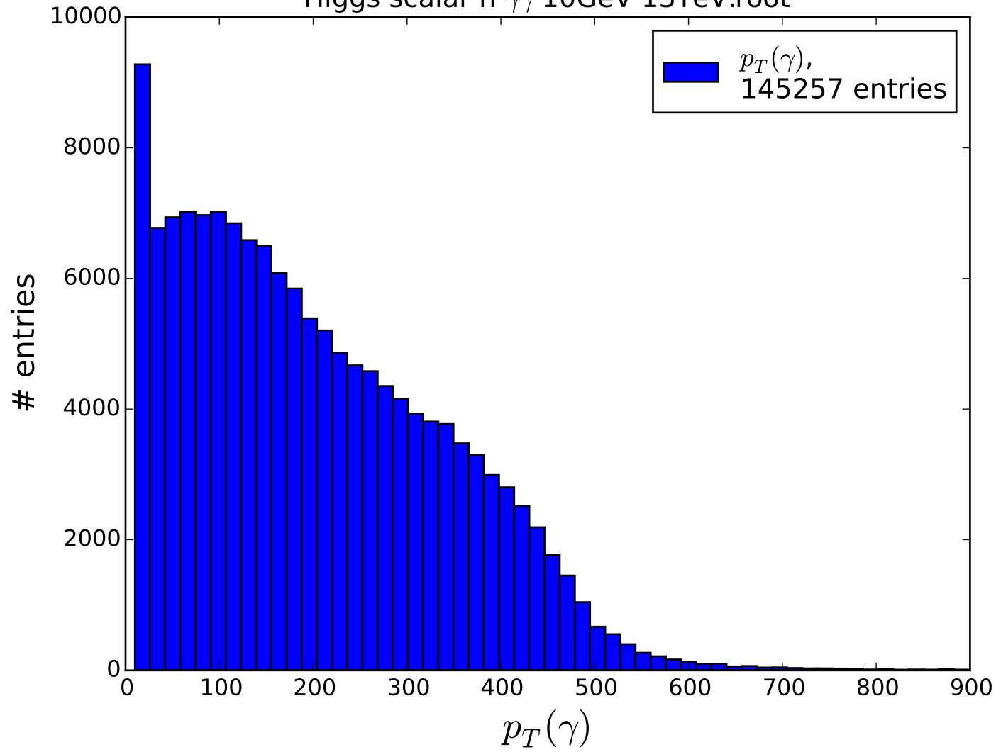
Higgs scalar h \rightarrow \gamma\gamma 10GeV 13TeV.root
