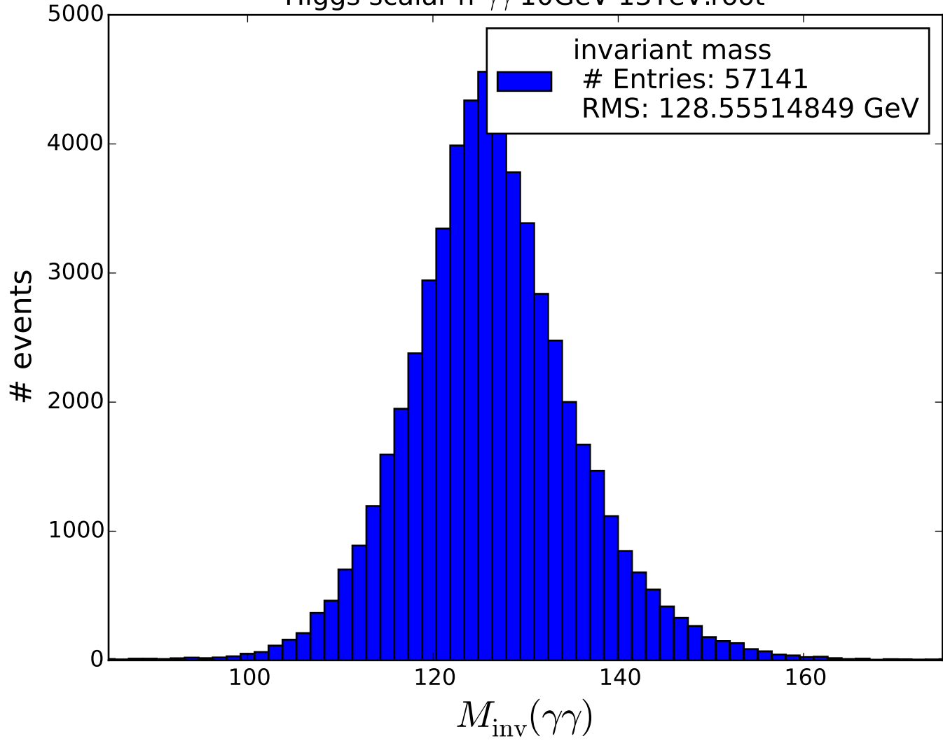
Higgs scalar h \rightarrow \gamma\gamma 10GeV 13TeV.root
